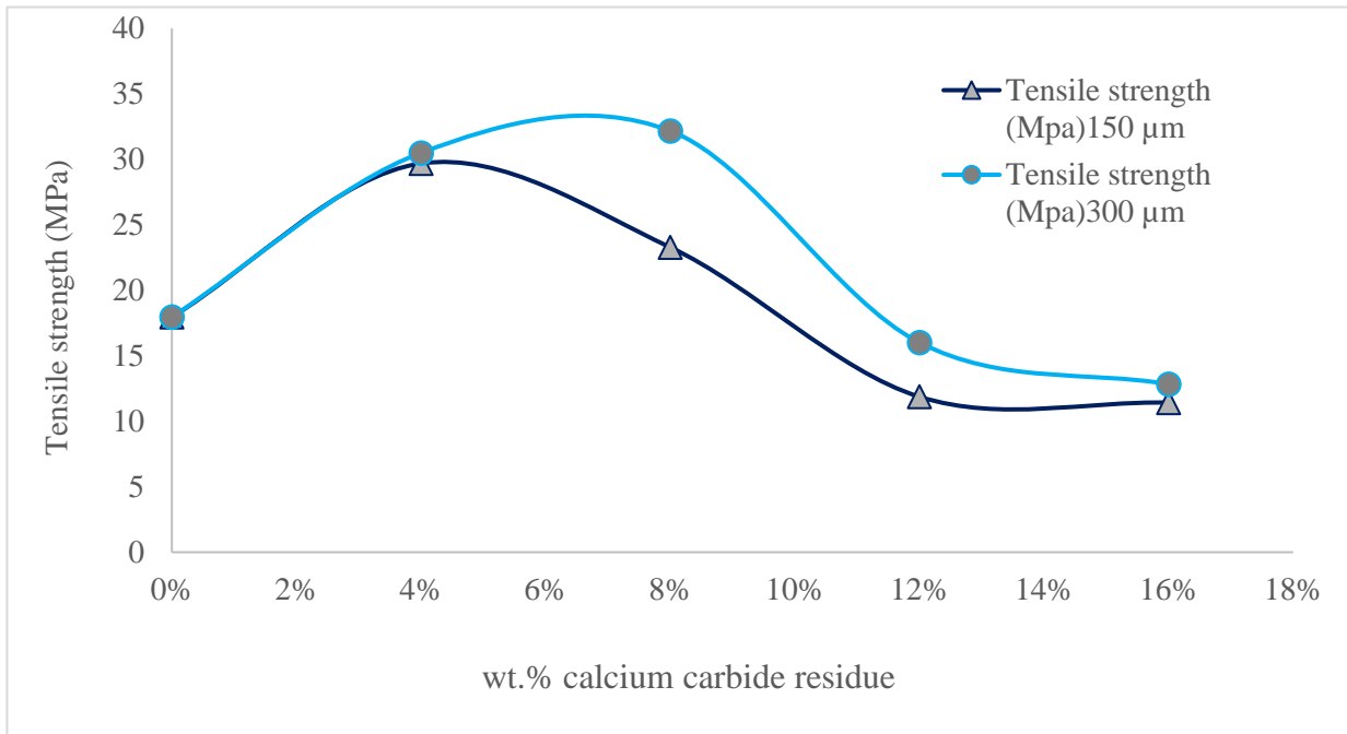
Figure 9: Plot of tensile strength against wt. % calcium carbide residue for composites produced using 150 and 300 μm particle sizes
