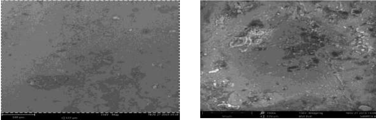
Figure 11 (a): SEM for 0 wt.% Calcium carbide residue (b): SEM for 4wt.% calcium carbide
