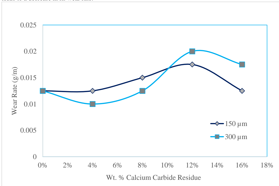
Figure 10: Plot of wear rate against wt. % calcium carbide residue for composites produced with 150 and 300 μm particle sizes
